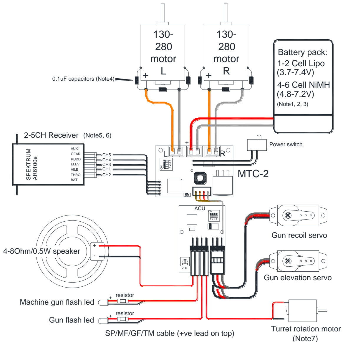
Fig.2 - Typical MTC-2 and ACU connection for tanks
