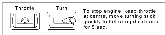
Engine stop by stick motion
