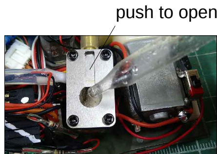
refill of smoke oil
